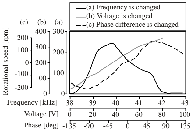
Fig. 3 Motor characteristics
