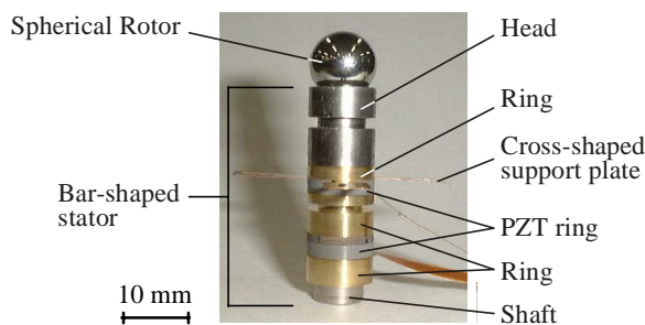
Fig. 2 The multi-DOF ultrasonic motor
