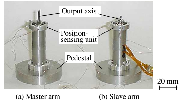
Fig. 5 Master and slave arms for active endoscope
