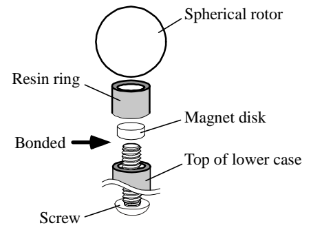
Fig. 8 Rotor/stator contact unit
