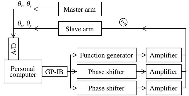
Fig. 9 Master-slave system
