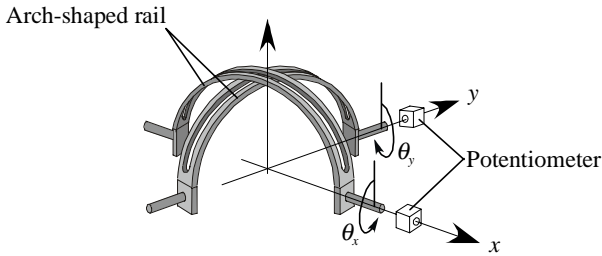
Fig. 7 Position sensing unit
