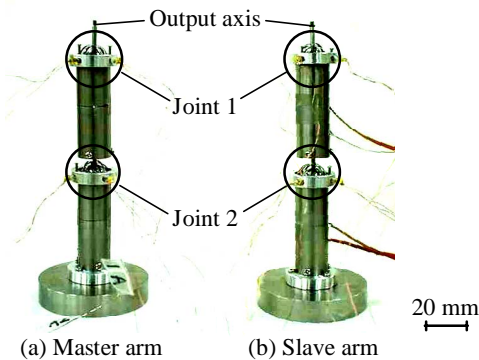
Fig. 11 Master and slave arms with two joints
