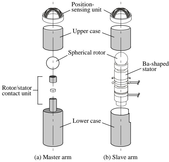
Fig. 6 Configurations of arms
