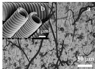
FIG. 1. (a) Optical microscopic image of CMCs/silicone-rubber composite. (b) SEM image of as-grown CMCs, showing the coils used with no gap.
